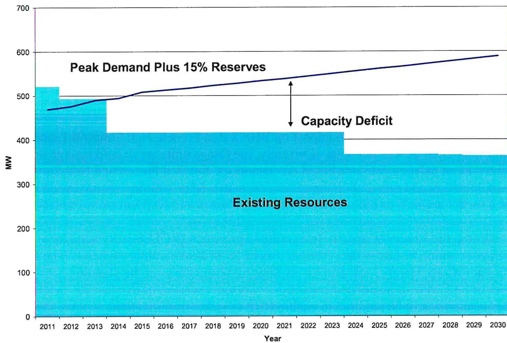
Figure 7.1 Black Hills Power Load and Resource Summary
